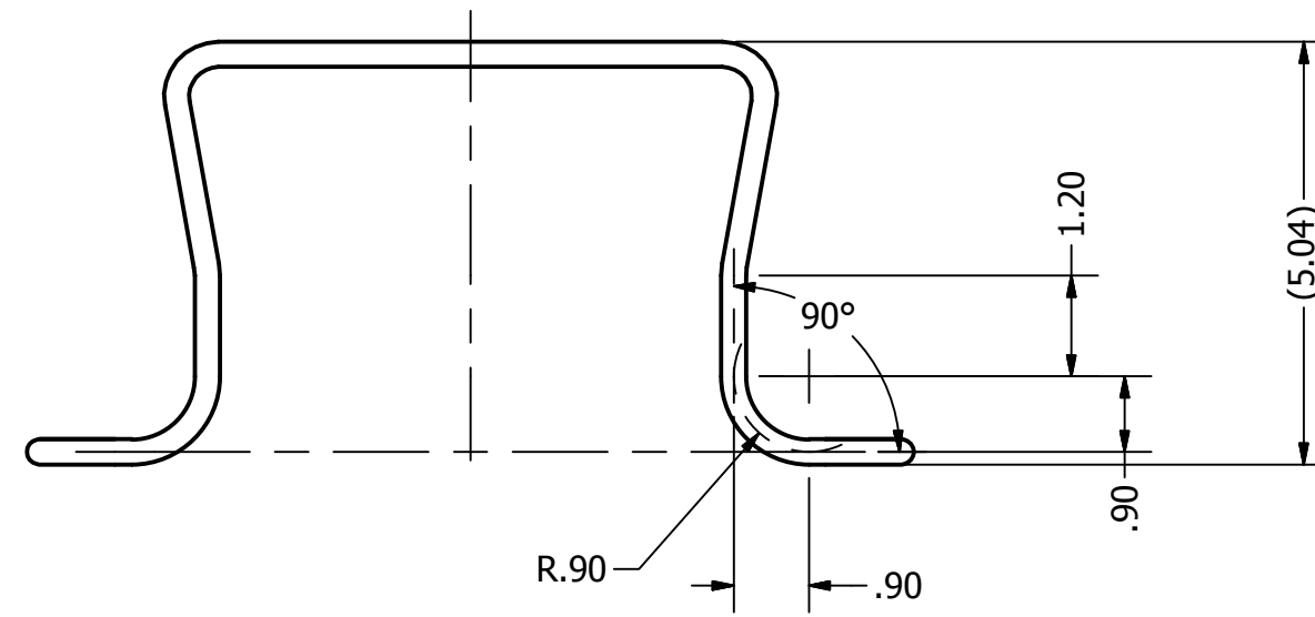
VIEW B-B
